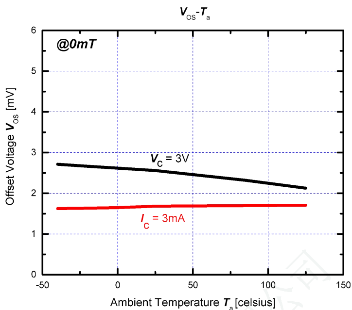
Figure 6. 非平衡电压-环境温度 Offset voltage V_{OS} as a function of ambient temperature T_a
